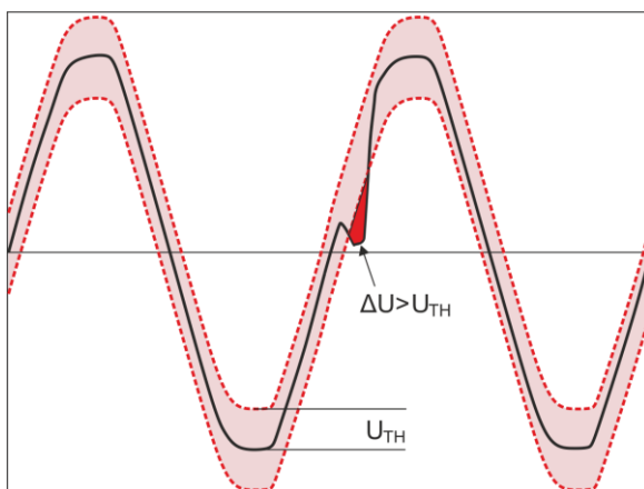
Fig. 42. Detecting waveshape variation events.
