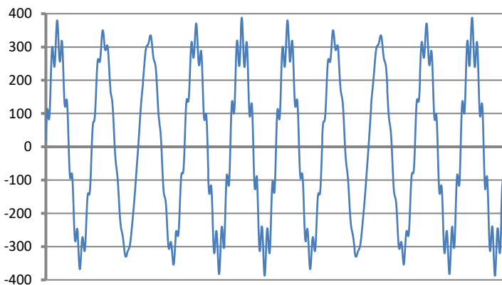
Fig. 47. The effect of 9th harmonic interaction (450 Hz, 10% U_{nom} ) and interharmonic 460 Hz (10% U_{nom} ). The apparent change in the voltage envelope with frequency of 10 Hz that may cause flicker ( U_{nom} = 230 V RMS, 50 Hz).
