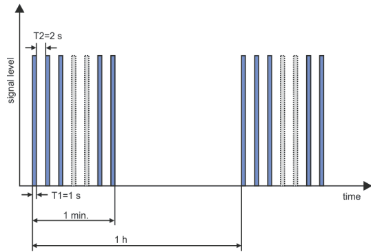
Fig. 48. An example of low-frequency signal transmission.
